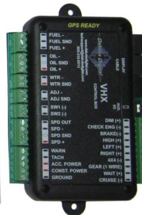
Control Box
