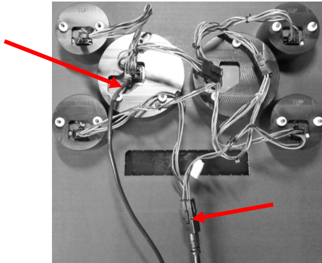
Buzzer Connector
