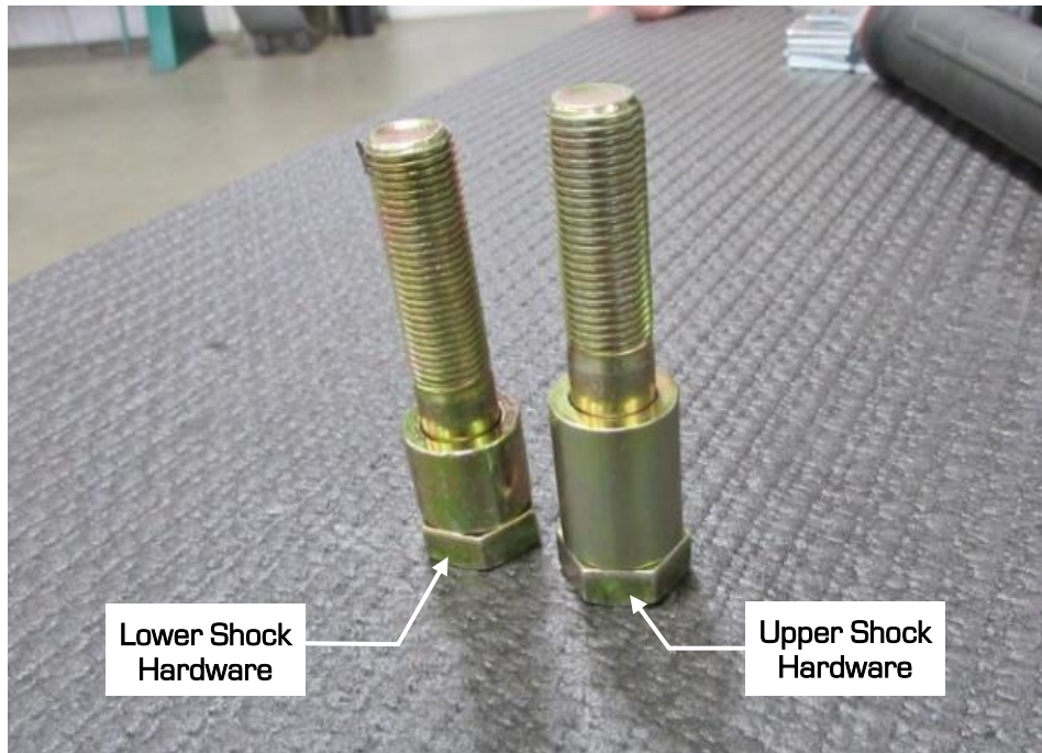
Figure 31 - Shock Mounting Bolts & Spacers
